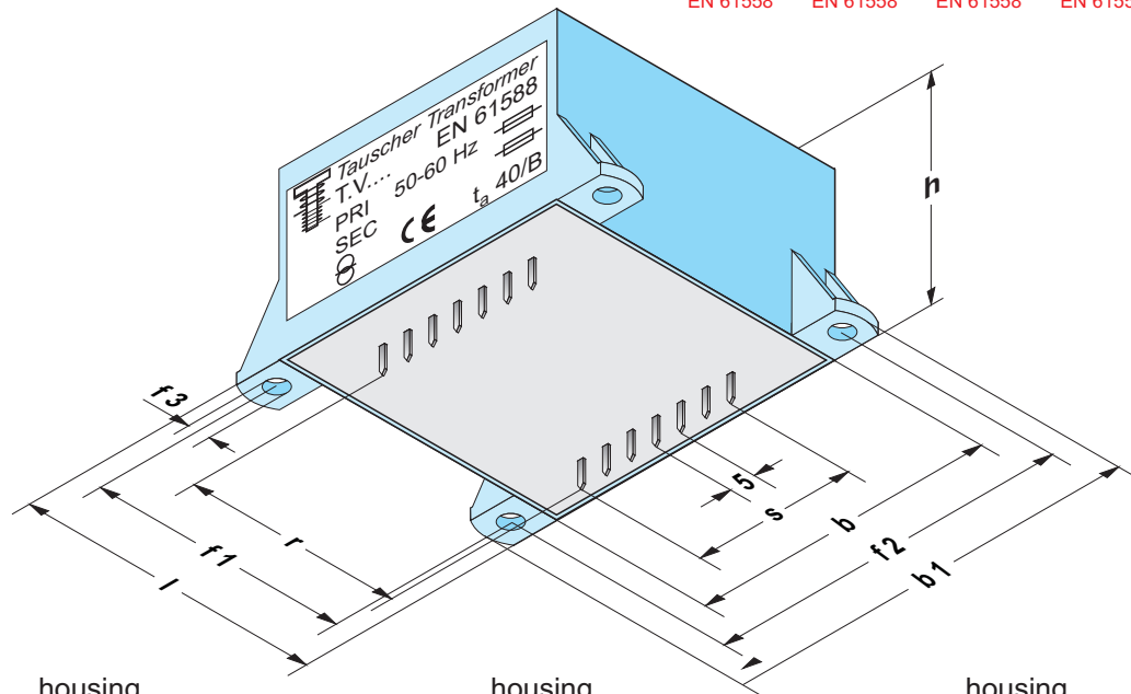
housing Gehäuse "0"
